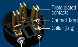
Triple plated contacts Contact Tang Collar (Lug) Combination Head slot and #2 Phillips
